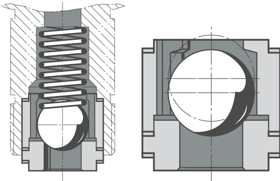
Ball valve
