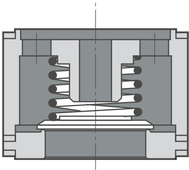
Disc valve
