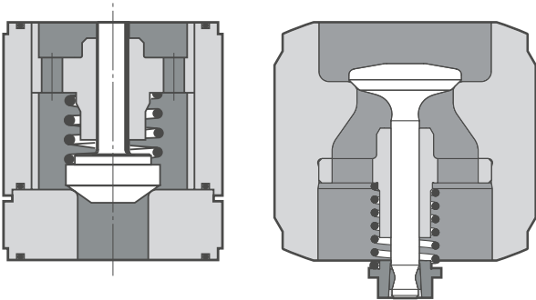
Cone valve
